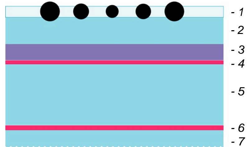
M-Jet micro encapsulation film - cross section
